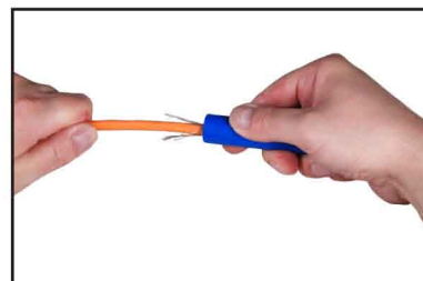
5. Put foil-shielded wires into „foil“ side of the tool
