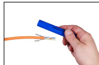
6. Cut foil shield by turning the tool, remove foil manually
